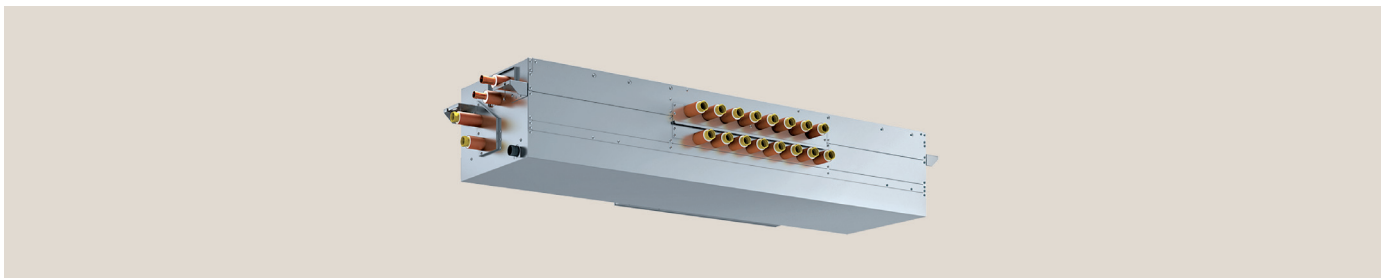
Abbildung 2.2 CMB-WP108V-G – HBC-Controller
